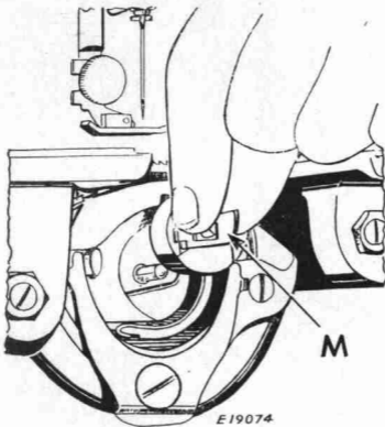
FIG. 7. REMOVING THE BOBBIN CASE
