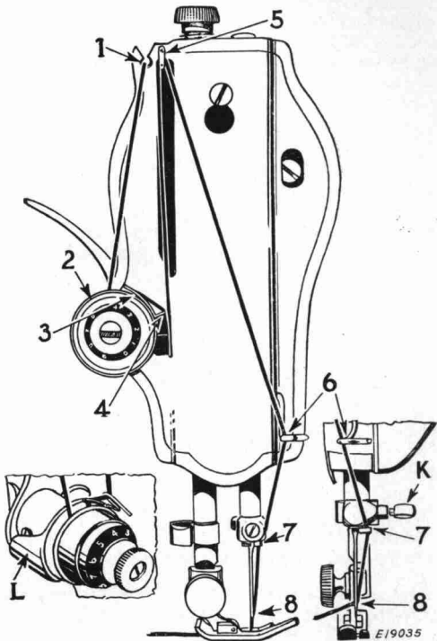
FIG. 6. UPPER THREADING
