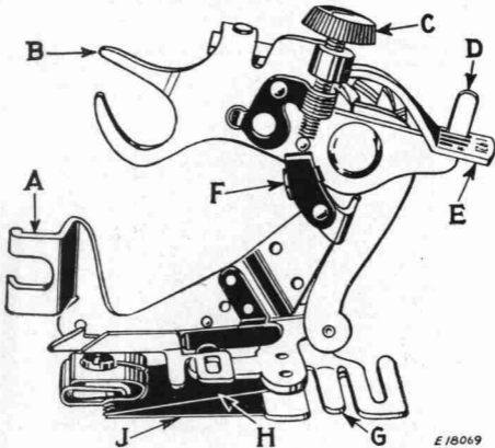
FIG. 60. PRINCIPAL PARTS OF THE RUFFLER
