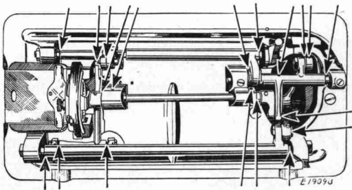
FIG. 28. OILING POINTS IN BASE OF MACHINE
