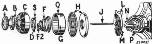
FIG. 22. NEEDLE THREAD TENSION DISASSEMBLED
