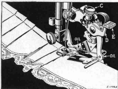
FIG. 71. GROUP PLAITING WITH THE RUFFLER
